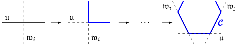
FIGURE 1. Bending hyperplanes into a crooked hyperplane.
