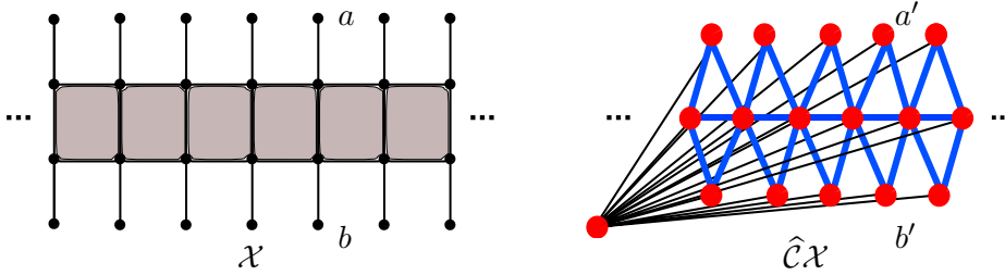
FIGURE 2. Cube complex drawn at left; its associated contact graph at right.
